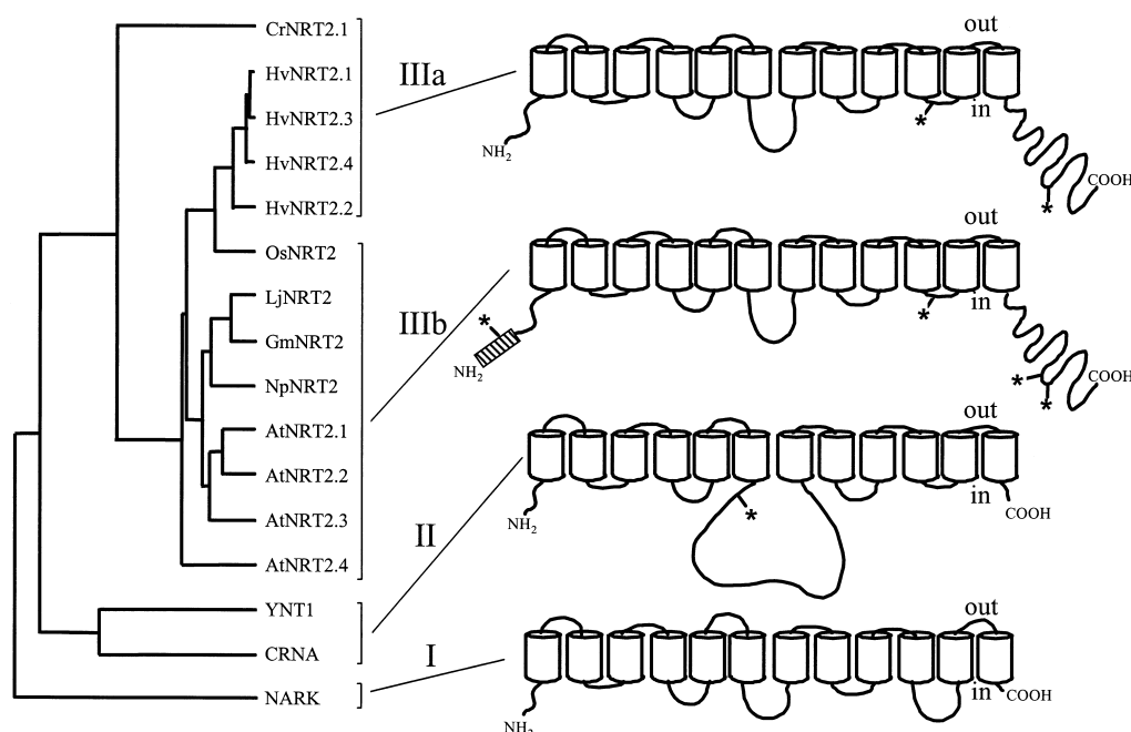
Fig. 2. Sequence relationships and comparisons of the predicted two-dimensional structures of members of the NNP family of \text{NO}_3^- and \text{NO}_2^- transporters. The amino acid sequences were aligned and the tree of sequence relationships generated using PILEUP [42] (only full-length sequences were used). See Table 1 for further details of the sequences used in the analysis and their GenBank accession codes. The diagrammatic representation of the membrane topologies of the transporters is based on previous predictions [21]. The domain indicated by a shaded rectangle represents a conserved N-terminal sequence that is specific to type IIIb NNP transporters. Asterisks indicate the location of conserved protein kinase C recognition motifs (S/T-x-R/K). The majority of the type IIIb sequences have two potential protein kinase C motifs within the C-terminal domain which are located nine amino acids apart (the exceptions being AtNRT2.1, which lacks the more C-terminal of the two motifs, and AtNRT2.2 which has neither). Amongst the type IIIa sequences, only the algal CrNRT2.1 and CrNRT2.2 [22] transporters have both motifs.
