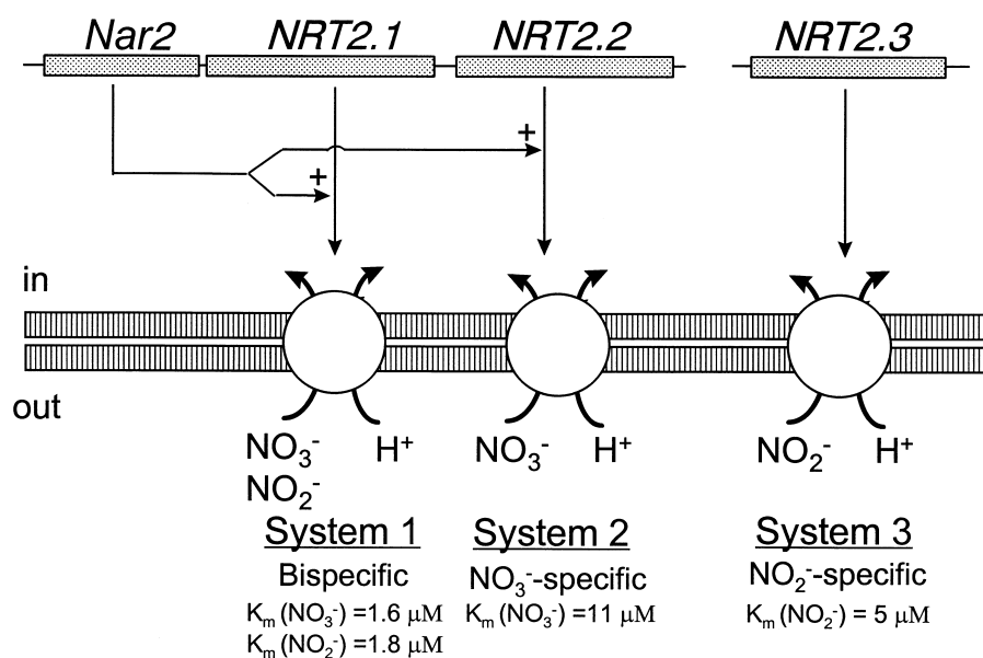
Fig. 1. Molecular genetics of the \text{NO}_3^- and \text{NO}_2^- transport systems in C. reinhardtii . The Nar2 gene which is closely linked to the NRT2.1 and NRT2.2 genes is required for the synthesis or activity of systems 1 and 2, but its precise function is unknown. The NRT2.3 gene which specifies system 3 is unlinked to the other three genes and does not have a requirement for Nar2 ; it is not known whether another Nar2 -related gene has a role in the biosynthesis of system 3. See text for further details.
