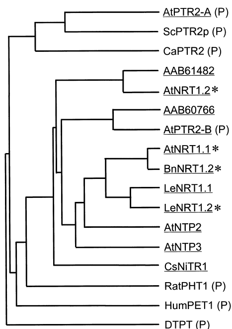
Fig. 4. Dendrogram showing sequence relationships between selected members of the PTR family. The amino acid sequences were aligned and the tree of sequence relationships generated using PILEUP [42]. Sequences indicated by an asterisk have been implicated in \text{NO}_3^- transport by functional analysis or by virtue of their \text{NO}_3^- -inducibility (see Table 1), while sequences known to be oligopeptide transporters are indicated by a (P). Plant sequences are underlined. Two of the plant sequences are known only by their GenBank accession numbers; the accession numbers of the other plant sequences can be found in Table 1. Accession numbers for the non-plant sequences are: ScPTR2 (P32901), CaPTR2 (P46030), RatPHT1 (BAA20489), HumPET1 (P46059) and DTPT (O07380).
