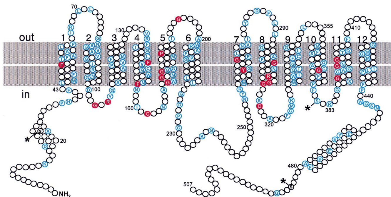
Fig. 3. Predicted membrane topology of HvNRT2.1. The assignment of the 12 predicted transmembrane domains was based on an analysis of multiply aligned HvNRT2.1, CrNRT2.1, CRNA and NARK sequences using the TMAP program [49], together with examination of the hydrophobicity profile of HvNRT2.1 [41] and comparisons with the experimentally determined topologies of other members of the MFS [44,45]. The topology and the boundaries of the transmembrane helices should not be considered as definitive but rather as a model which needs to be experimentally verified. Residues conserved in an alignment of all the bacterial, fungal, algal and plant sequences in Fig. 2 are indicated in red and residues conserved in all the plant and algal sequences in blue. Three serine residues which are located within conserved protein kinase C motifs are marked by asterisks: Ser-28 is part of a S/T-x-R motif found in all HvNRT2 sequences and in OsNRT2; Ser-381 (between transmembrane helices 10 and 11) is part of a S-x-R motif found in all the plant and algal sequences; Ser-484 (in the C-terminal domain) is part of a S-x-R motif found in the algal and the majority of the higher plant sequences. Two regions of predicted \alpha -helix which appear to be conserved in similar locations in the hydrophilic N- and C-terminal domains of other higher plant NRT2 polypeptides are also shown.
